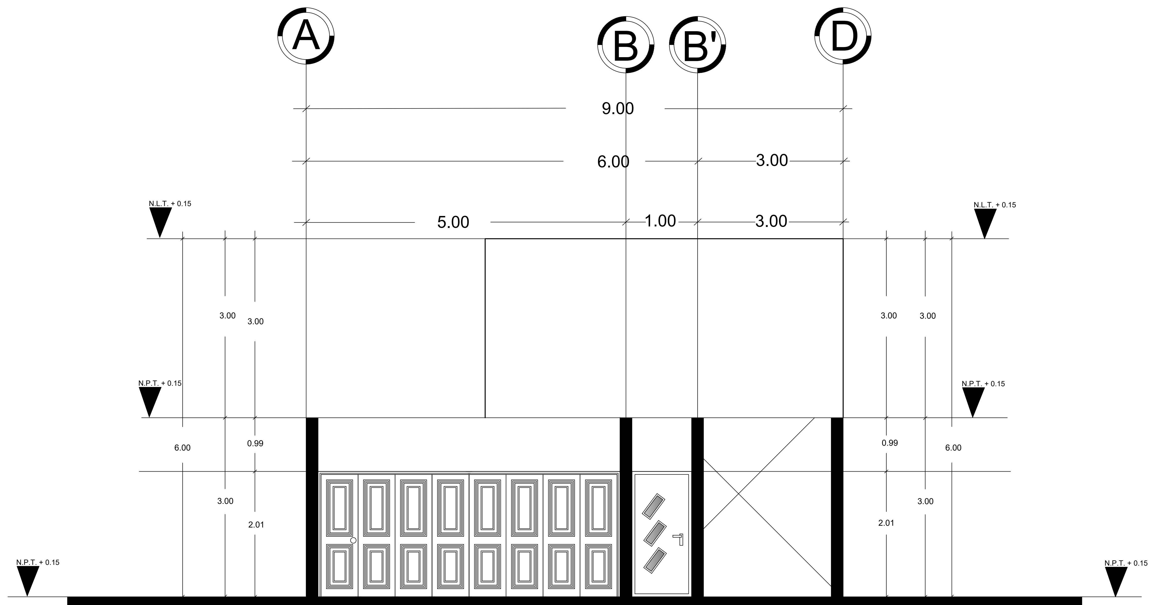
FACHADA PRINCIPAL ESC: 1:50
