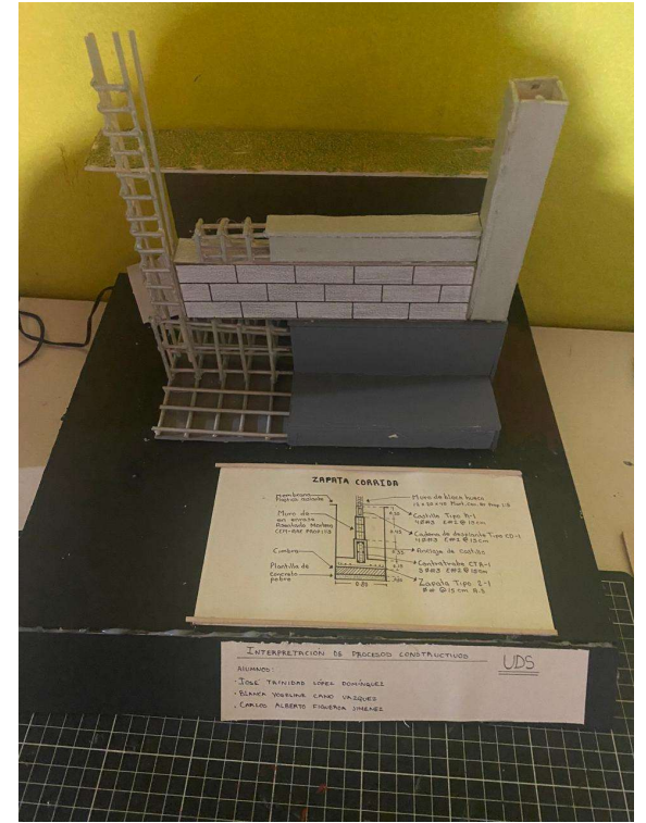
ZAPATA CORRIDA
