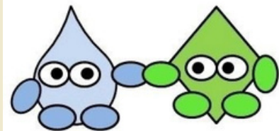
adhesion
