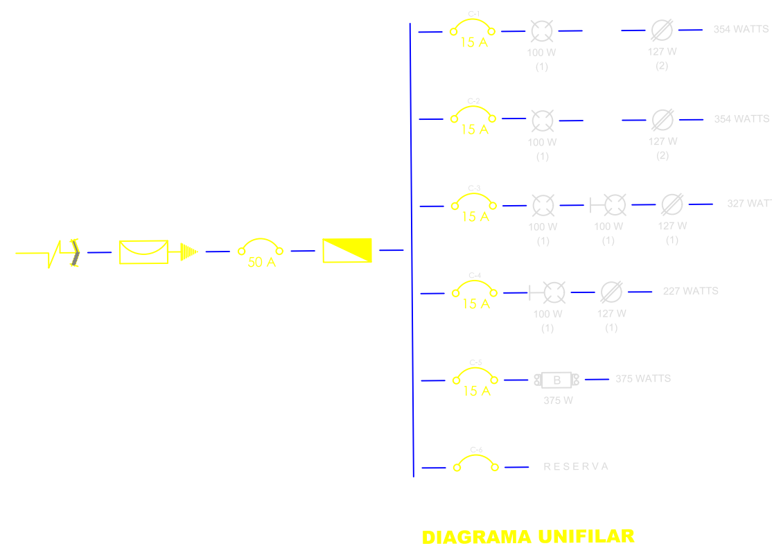
DIAGRAMA UNIFILAR
