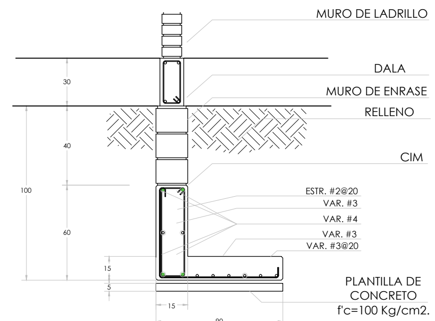
ZAPATA COLINDANTE INTERIOR ZC-3
