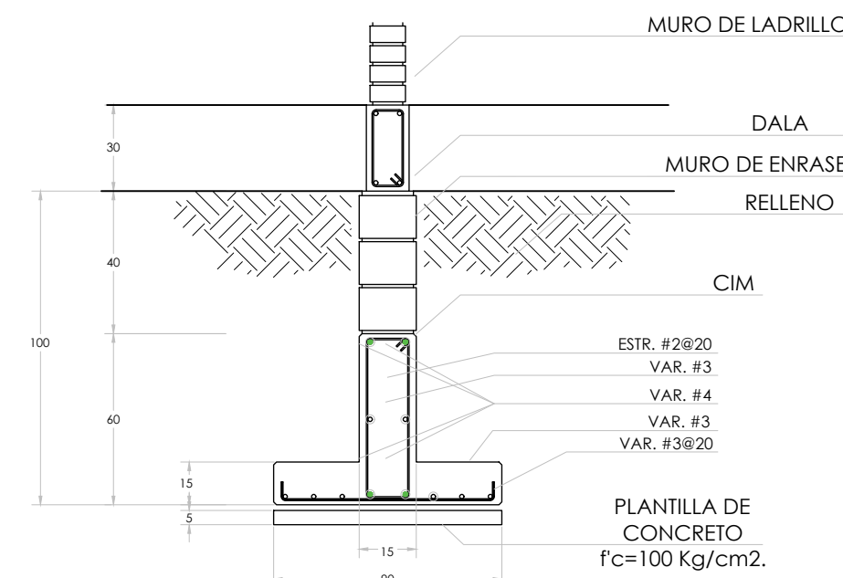
ZAPATA CORRIDA INTERMEDIA ZC-2
