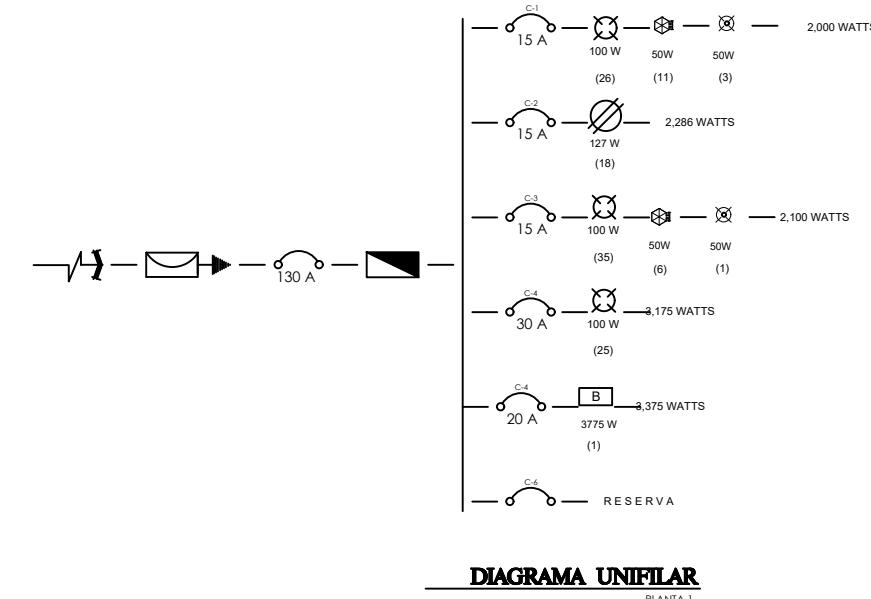
DIAGRAMA UNIPOLAR
