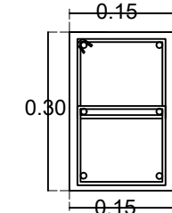
K-3 15X30X0.01=4.5 4 var. #4-2 Var.#3 Est. #2 @15 cm Doble
