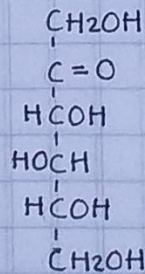
D-sorbosa
