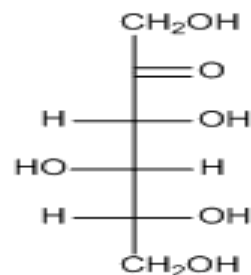
D-(+)-Sorbosa
