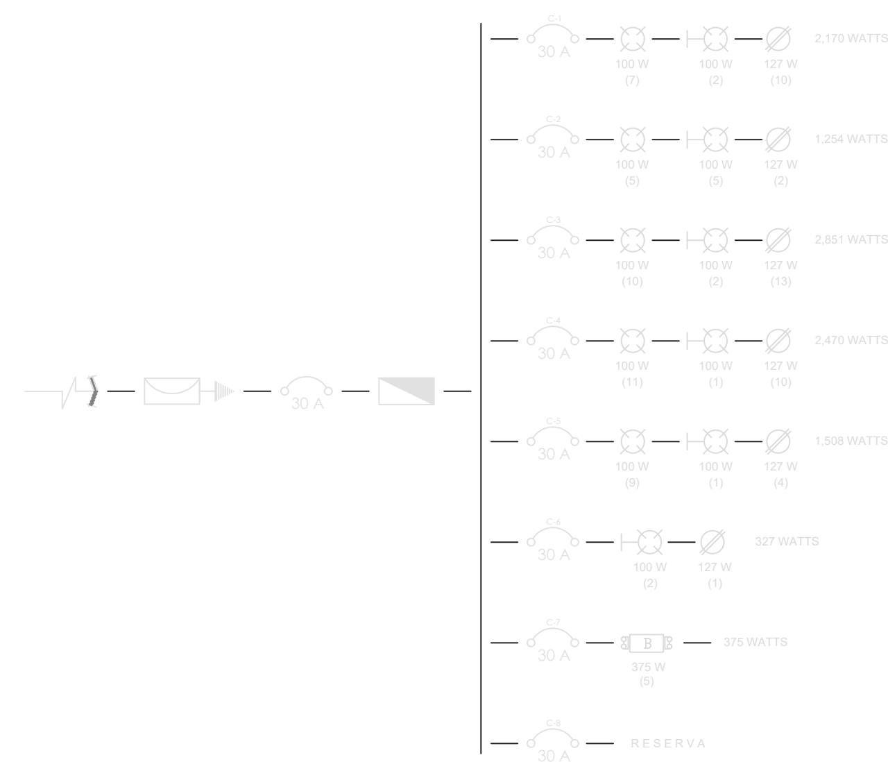
DIAGRAMA UNIFILAR
