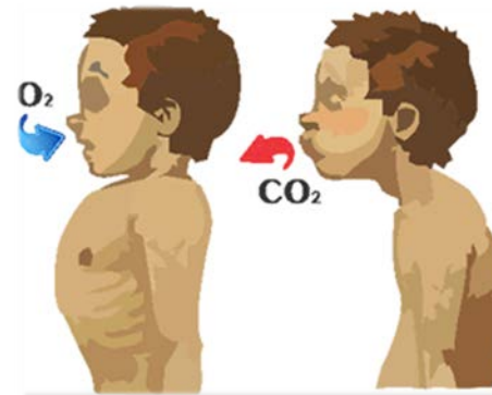
Breathing frequency
