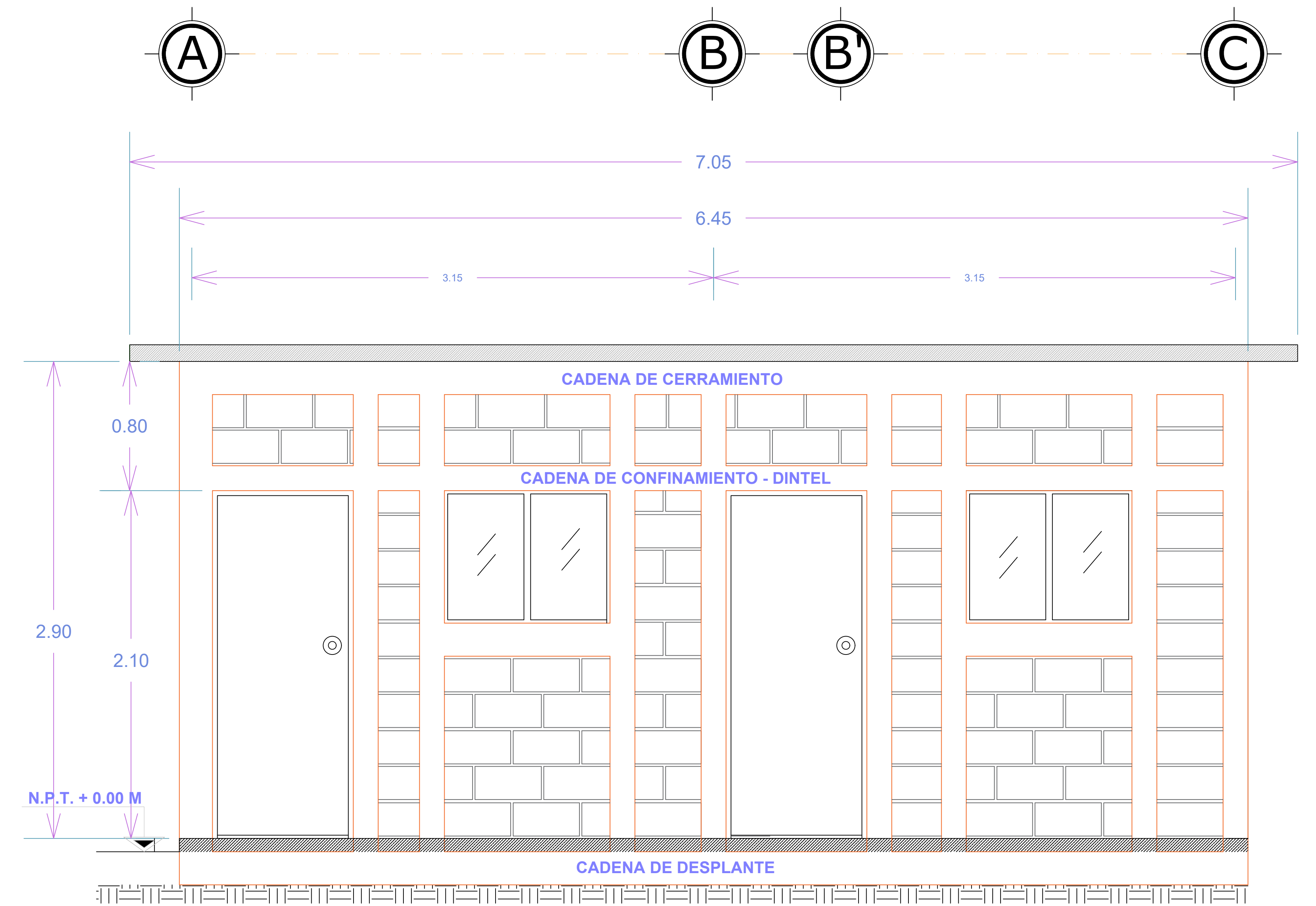
FACHADA PRINCIPAL
