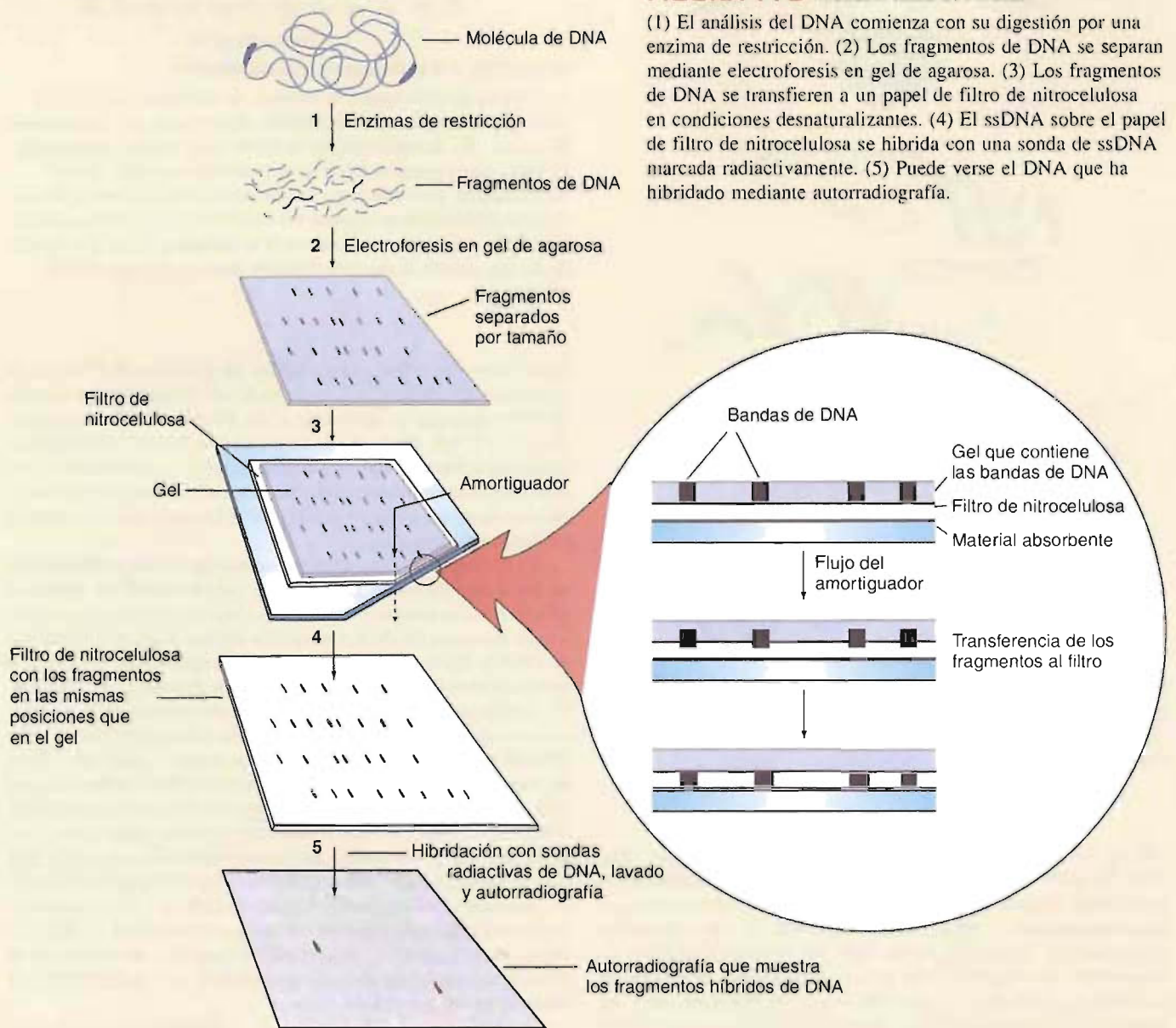
FIGURA 17D Transferencia Southern.
