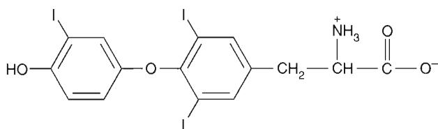
Triyodotironina ( T_3 )
