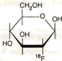
2-Desoxi-2-[ 18 F] fluoro-β-D-glucosa
