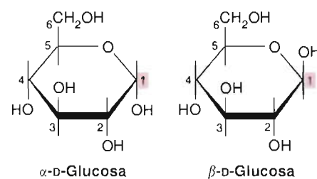
(a) \alpha -D-Glucosa (b) \beta -D-Glucosa
