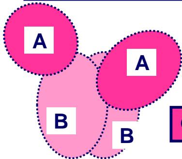
GyrB/ParE
